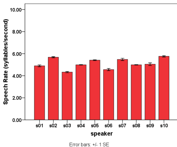
Figure 4: Individual variation of speech rate which is calculated as the number of syllables per second.
