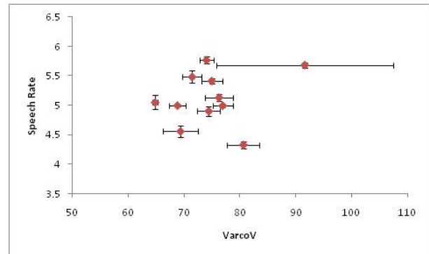
Figure 5: Plot of mean values with standard errors for acoustic parameters of VarcoV and Speech Rate. The whiskers indicate one standard error (i.e. +/-1 SE).
