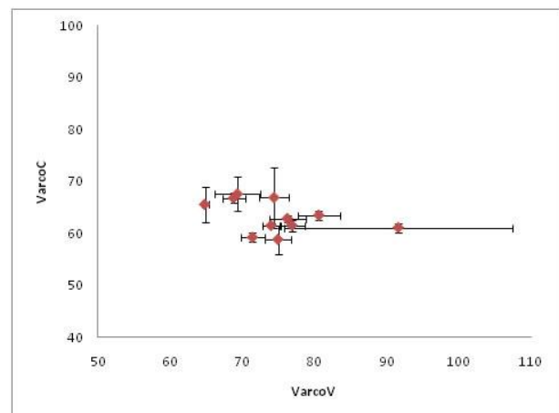
Figure 6: plot of mean values of VarcoV and VarcoC. VarcoC, centring around 62-65 appear to exhibit less degree of both inter- and intra-speaker variability than VarcoV in the Buckeye corpus.
