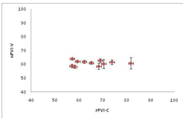
Figure 7: Plot of mean values of rPVI-C and nPVI-V. nPVI-V, proposed in [4], shows quite a consistent pattern across speakers. rPVI-C, proposed in [3], on the other hand, does not function well enough to capture between-speaker invariability.
