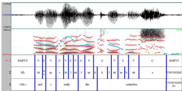
Figure 1: Screenshot of the segmentation of phone-labeled spoken utterances into consonant (C) and vocalic (V) intervals (1 st tier), phone and word transcription (2 nd and 3 rd tiers, respectively). The phone and word transcription are provided. A script is written that converts the phones into consonants and vowels, and generates automatically the CV sequence as shown in the 1 st tier.
