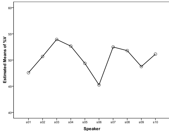
Figure 3: Individual variation of the proportion of the vocalic duration as calculated as %V.
