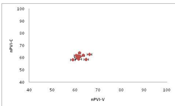
Figure 8: Plot of mean values of nPVI-V and nPVI-C. Both measures show the least inter-speaker and intra-speaker variation.
