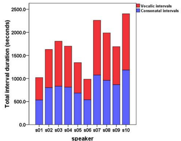
Figure 2: Individual variation of the total interval duration and the ratio of consonantal interval and vocalic intervals.
