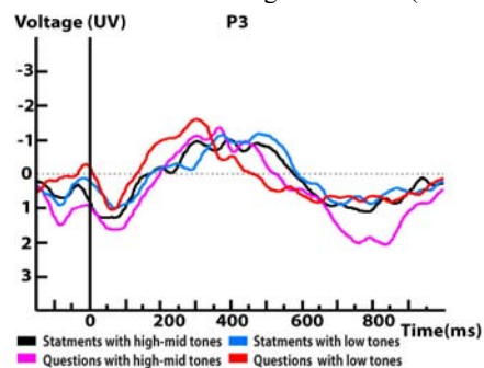
Figure 1: Grand average waveforms for electrode P3 time-locked to the onset of the sentence-final critical word in Experiment 1.
