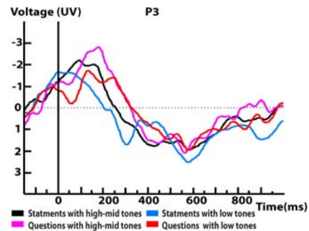
Figure 2: Grand average waveforms for electrode P3 time-locked to the onset of the sentence-final critical word in Experiment 2.
